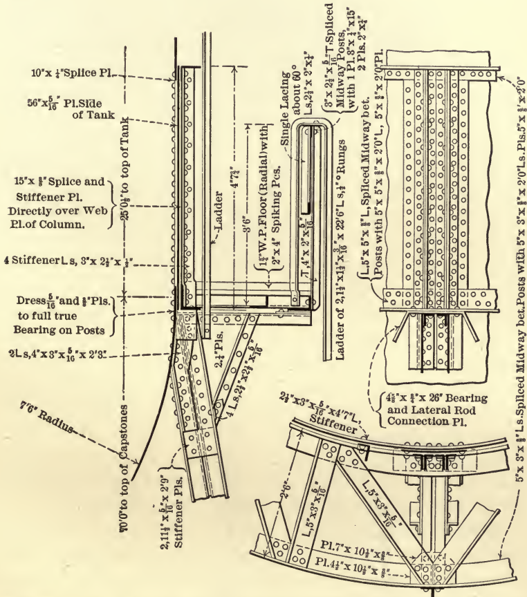
FIG. 56.—Detail of Junction Between Sides and Bottom of Elevated Steel Tanks. (Designed by Prof. A. Marston.)
